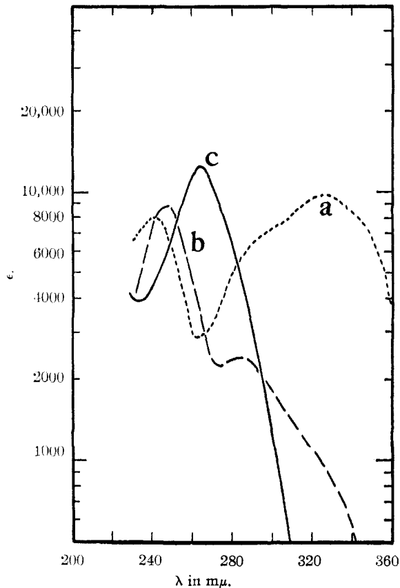
Fig. 4.—Absorption spectra: a, C_6H_5COCH=CHONa ; b, C_6H_5COCH_2CHO ; c, C_6H_5COC\equiv CH ; solvents: a and c, 95% EtOH; b, 0.01 N HCl; maxima: a, 240 and 327 m\mu ; b, 247 and 284 m\mu ; c, 264 m\mu .
